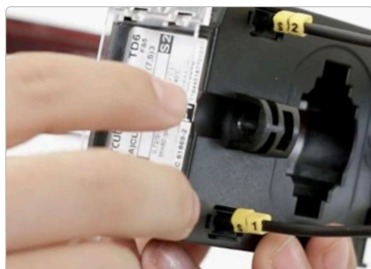
Terminal cover disables access to fastening screws and product label.
